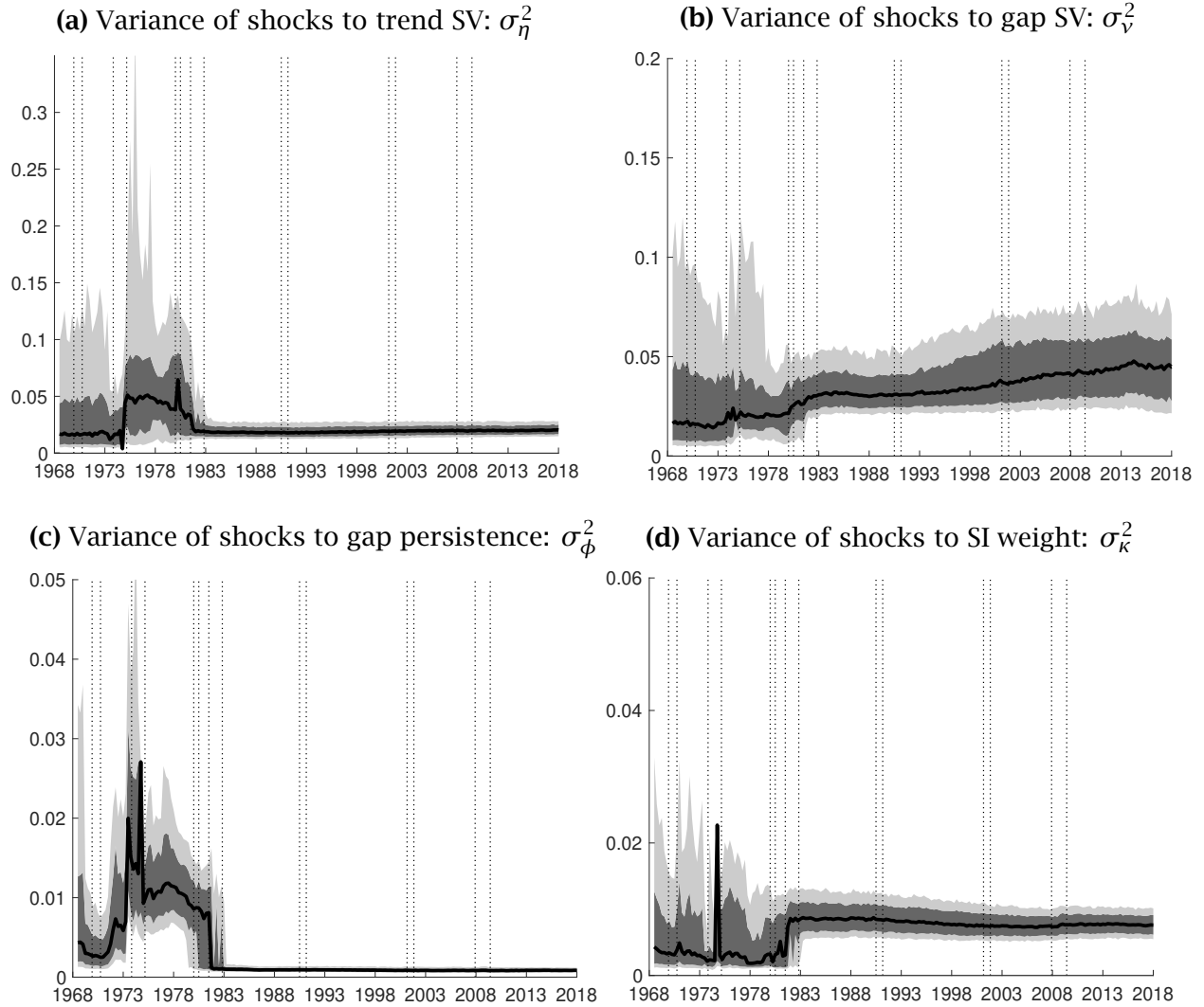
Figure 2: PARTICLE LEARNING FILTER ESTIMATES OF STATIC PARAMETERS
