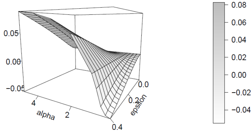
Average(|d1_R-theta1|-|d1_RN-theta1|)
