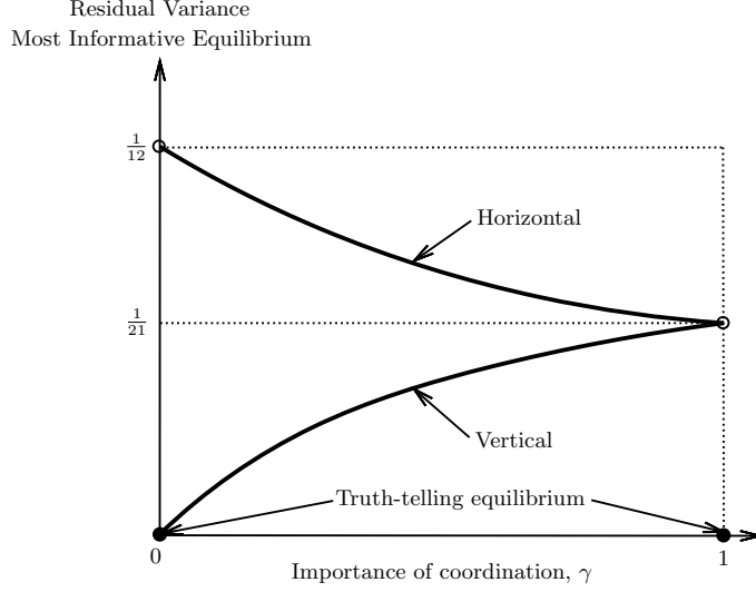
Figure 1: Predicted communication quality as a function of \gamma .
