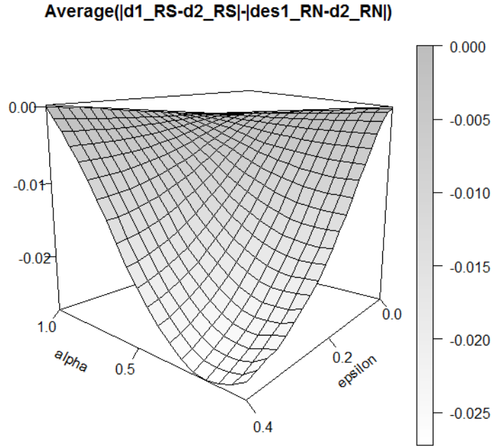
(a) Comparison of average distances between optimal risk-seeking and risk-neutral decisions, |d_1^{RS} - d_2^{RS}| - |d_1^{RN} - d_2^{RN}| for \gamma = \frac{1}{4} . Each point corresponds to the average over (\nu_1, \nu_2) \in [-0.6, 0.6]^2 with a grid of size 0.05. The grid size for \alpha is 0.05.
