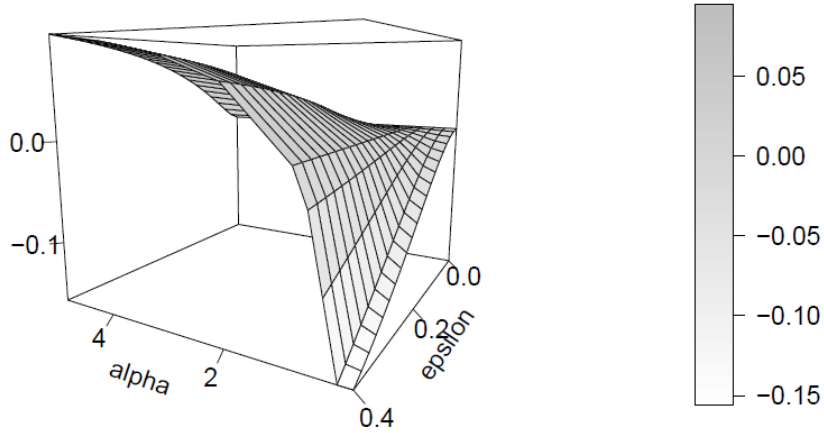
Average(|d1_R-theta1|-|d1_RN-theta1|)
