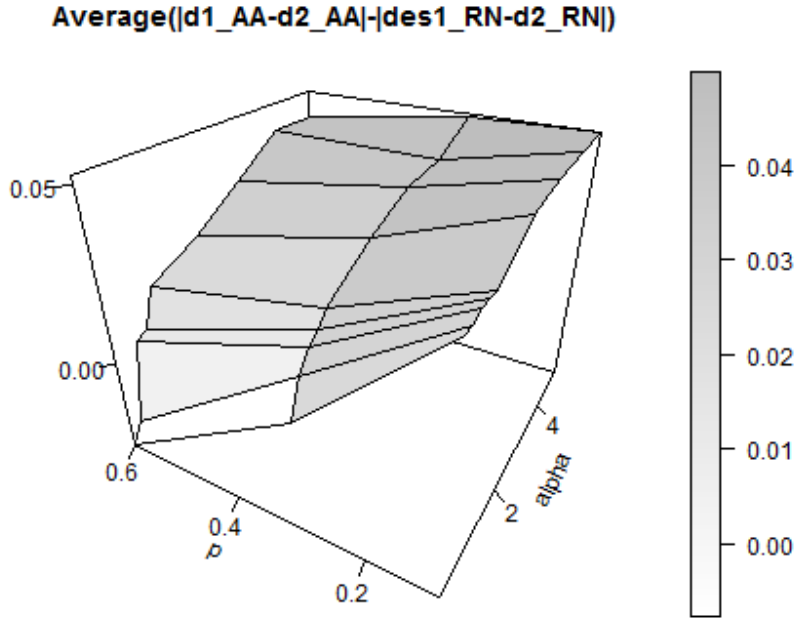
(a) Comparison of average distances between optimal maxmin and risk/ambiguity-neutral decisions, |d_1^{AA} - d_2^{AA}| - |d_1^{RN} - d_2^{RN}| for \gamma = \frac{1}{4} , different degrees of risk aversion \alpha , and different distribution parameters p . Each point corresponds to the average over (\nu_1, \nu_2) \in [-0.6, 0.6]^2 with a grid of size 0.05. The grid size for the decisions is 0.05, and the value of \epsilon = 0.4 .
