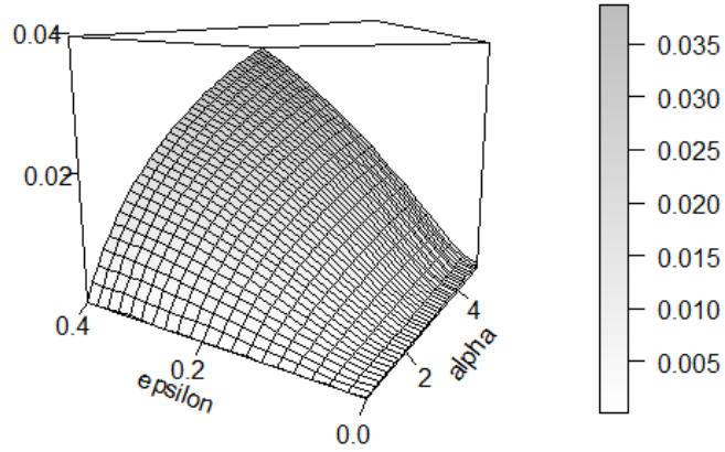
(b) Comparison of average distances between optimal risk-averse and risk-neutral decisions, |d_1^{RA} - d_2^{RA}| - |d_1^{RN} - d_2^{RN}| for \gamma = \frac{3}{4} . Each point corresponds to the average over (\nu_1, \nu_2) \in [-0.6, 0.6]^2 with a grid of size 0.05.
