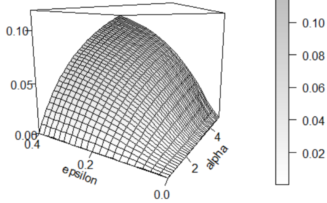
(a) Comparison of average distances between optimal risk-averse and risk-neutral decisions, |d_1^{RA} - d_2^{RA}| - |d_1^{RN} - d_2^{RN}| for \gamma = \frac{1}{4} . Each point corresponds to the average over (\nu_1, \nu_2) \in [-0.6, 0.6]^2 with a grid of size 0.05.
