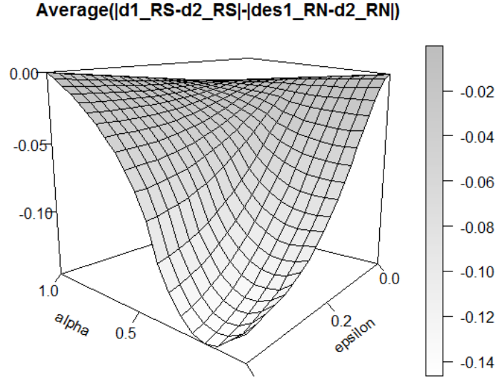
(a) Comparison of average distances between optimal risk-seeking and risk-neutral decisions, |d_1^{RS} - d_2^{RS}| - |d_1^{RN} - d_2^{RN}| for \gamma = \frac{1}{4} . Each point corresponds to the average over (\nu_1, \nu_2) \in [-0.6, 0.6]^2 with a grid of size 0.05. The grid size for \alpha is 0.05.
