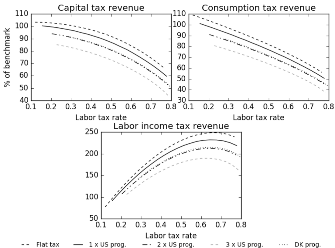
Figure 4: The Impact of Tax Progressivity on Revenue From Labor Income Taxes, Consumption Taxes and Capital Income Taxes
