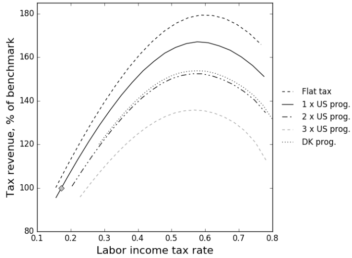
Figure 6: The Impact of Tax Progressivity on the s-Laffer Curve (wasting additional revenue)
