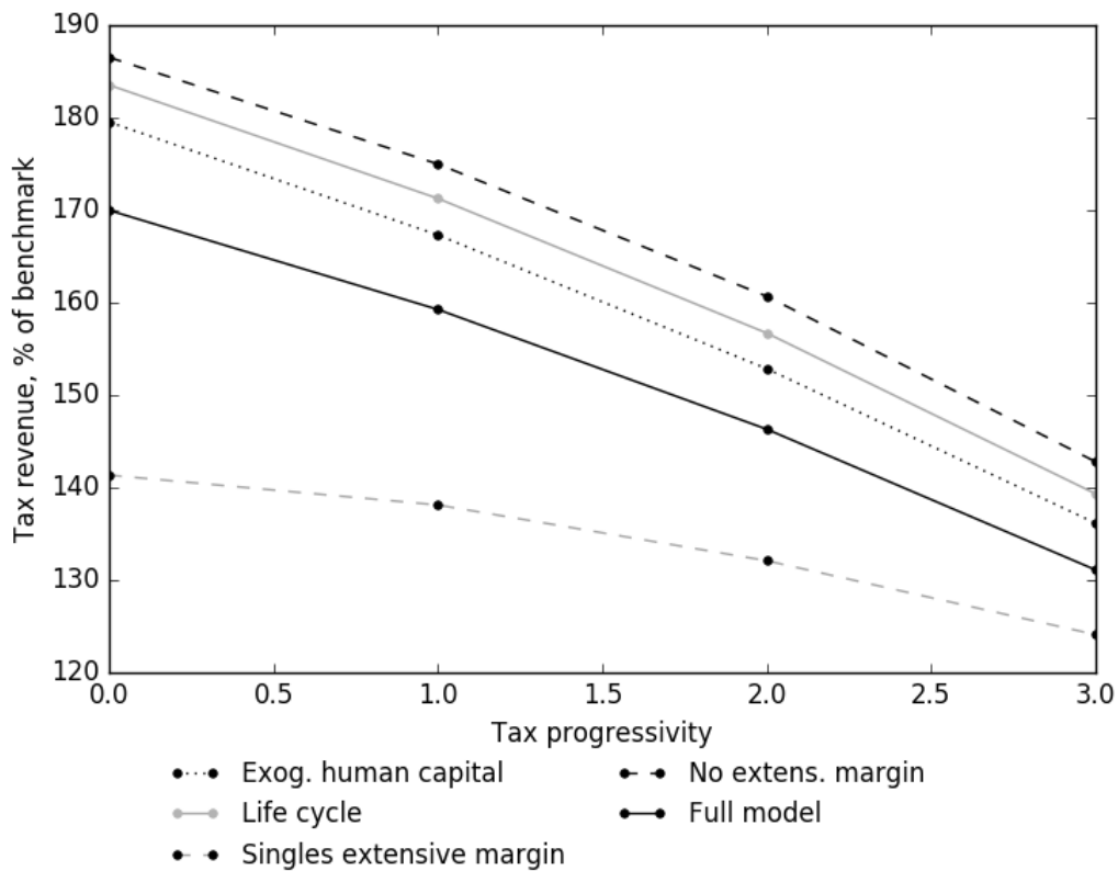
Figure 7: The Impact of Tax Progressivity on Maximum Revenue in Different Models
