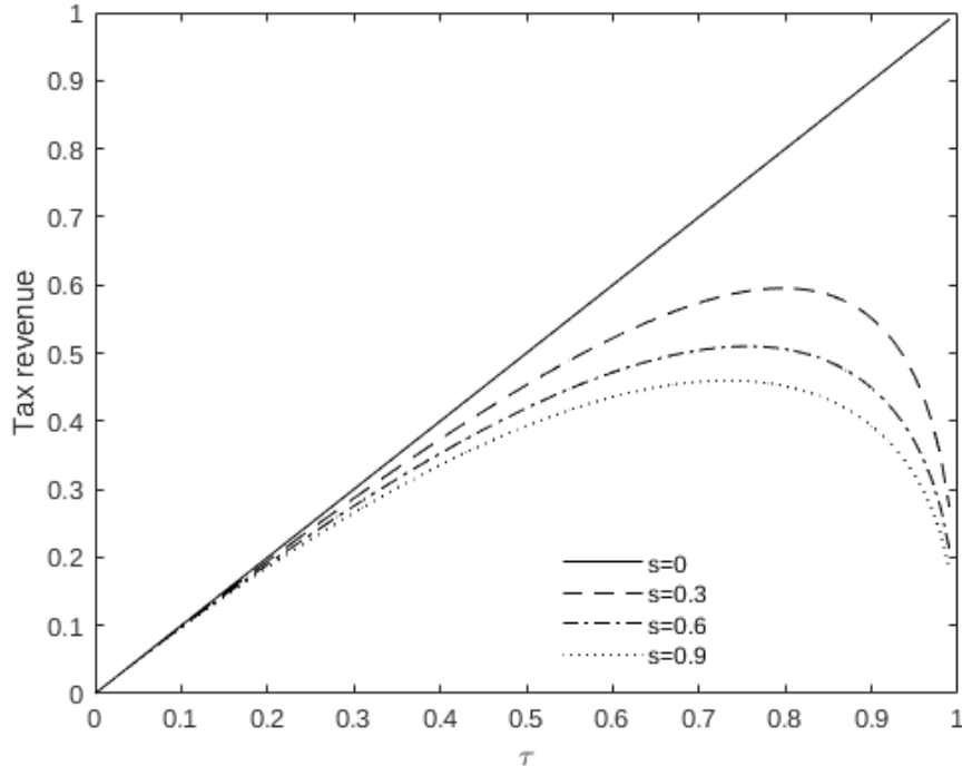
Figure 1: The Laffer Curves in a Static Model with a Representative Household for Different Values of s
