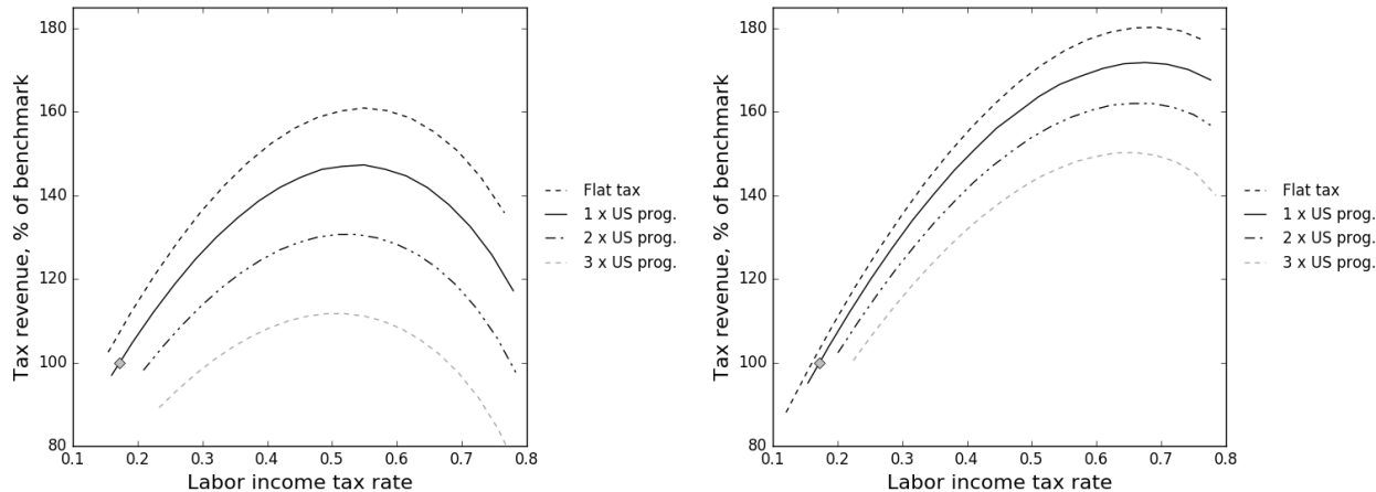
Figure 2: Laffer Curves by Tax Progressivity, High (left panel) and Low (right panel) Intensive Margin Labor Supply Elasticity
