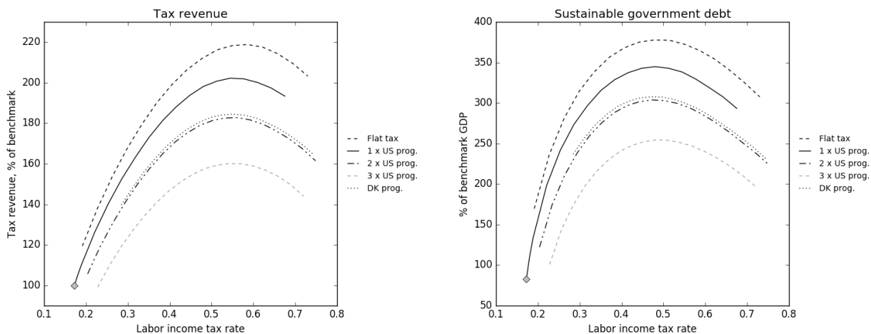
Figure 5: Tax Revenue and Maximum Sustainable Debt Level by Tax Level and Progressivity
