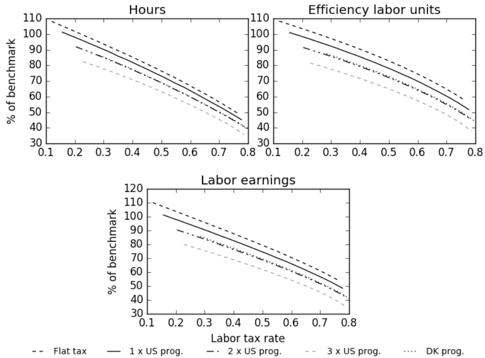
Figure 3: Labor Supply and Earnings Statistics by Tax Progressivity and Level for g-Laffer Curves
