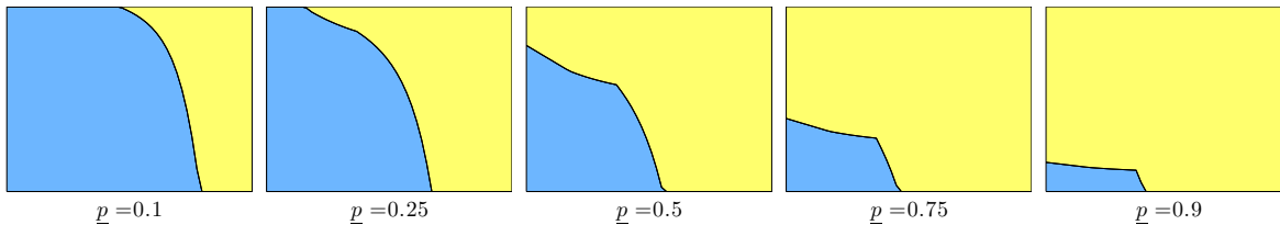
Figure 2: Example breakdown frontiers for the claim \mathbb{P}(Y_1 > Y_0) \geq p , for five different values of p .
